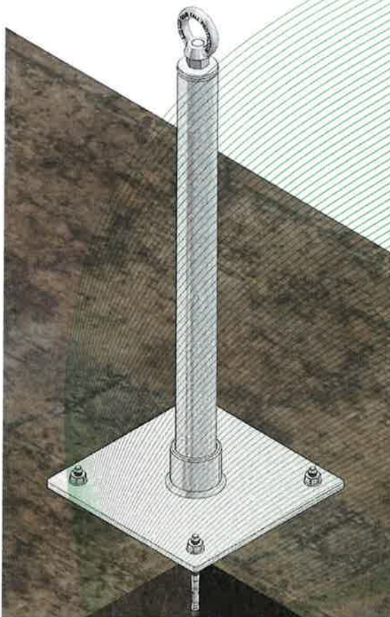
Fig. 1: Anchor device, type: LUX-top® Abseilpunkt (mounting example)
